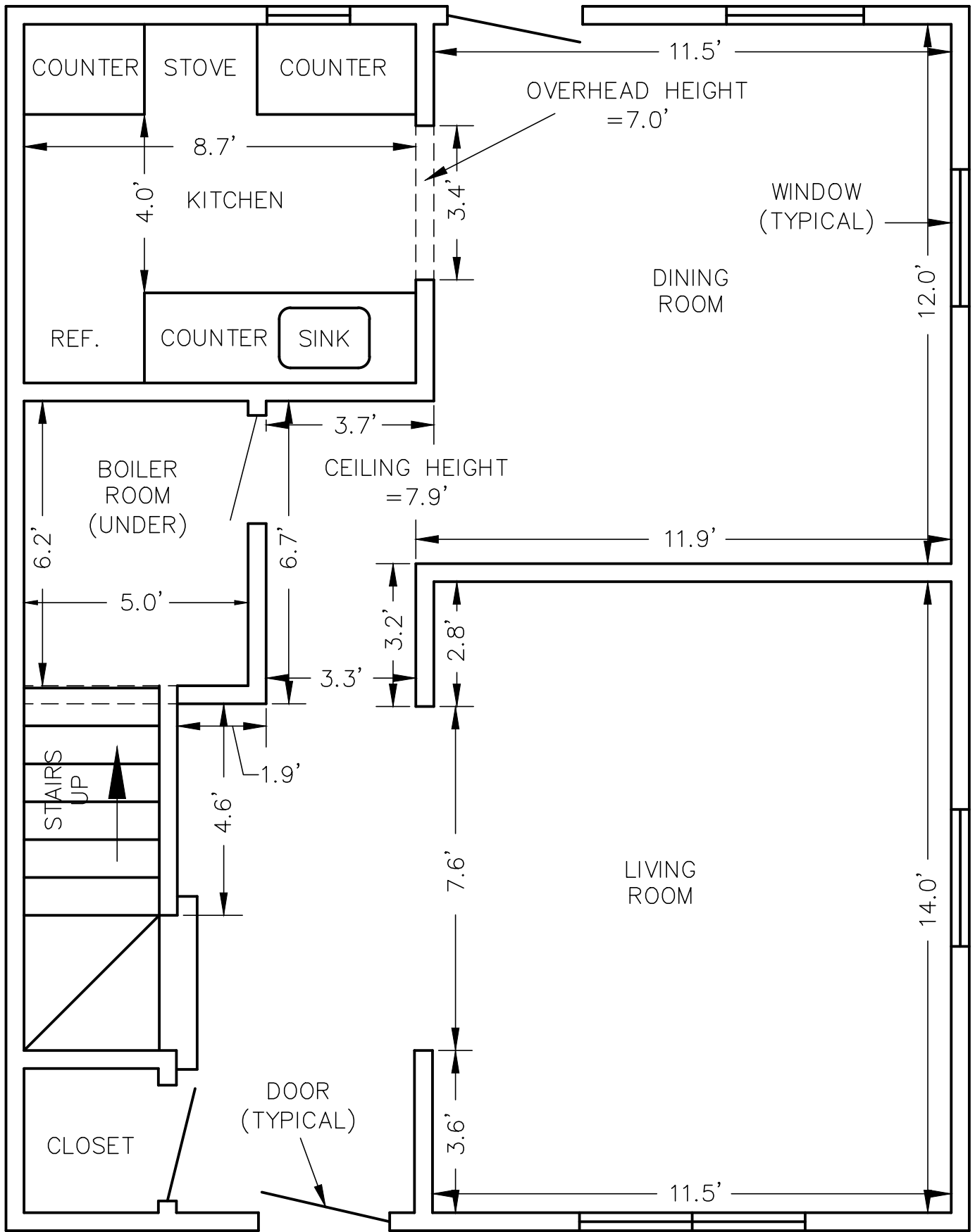
PHEASANT COURT (1ST FLOOR)
